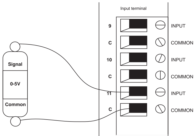
Figure 8: 0-5V sensor
